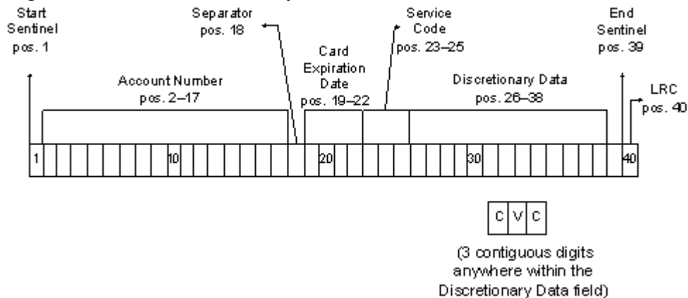
Figure A.3—Track 2 Data Layout
